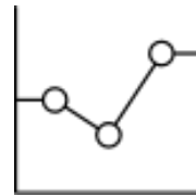
Data Science
