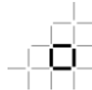
Blockchain
